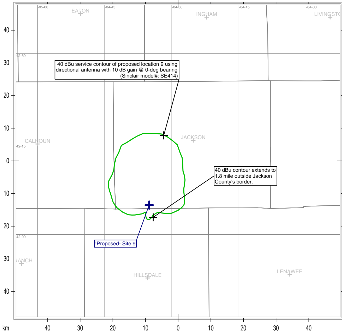
40 dBu service contour of proposed location 9
